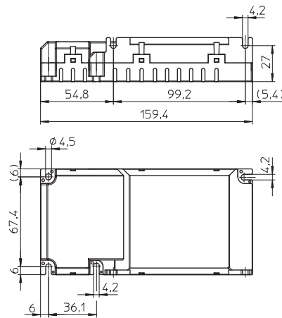
K3 with cord grip
