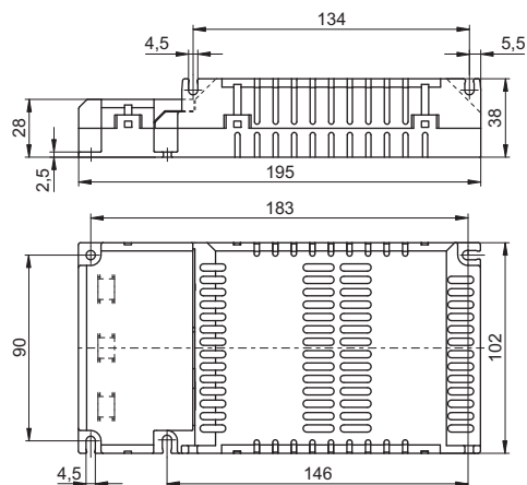
K4+ with cord grip and venting slits
