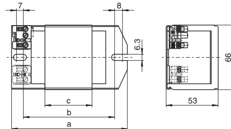
A Push-in terminals: 0.5-1.5 mm 2
