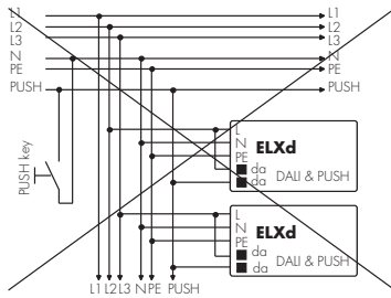
Fig. 1 N conductor must not be used as a PUSH potential
