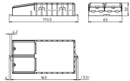
K34 with cord grip
